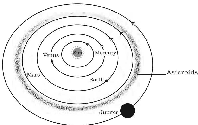
Fig. 17.25 : Asteroid belt
