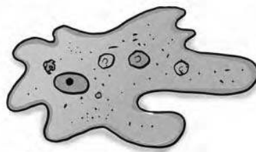
Amoeba
