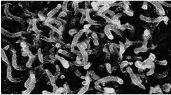
Spiral bacteria
