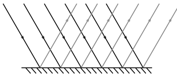
Fig. 16.8 : Regular reflection
